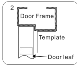
2 Close the door first, then place the upper side of template on door frame, while adjust the left side next to the door leaf. Hollow Metal Door Wooden Door Metal Surface Door
