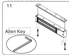
11 Use Allen key to screw the lock body on the mounting plate.
