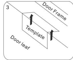
3 Mark screw positions of armature plate and magnetic lock on door leaf and door frame respectively.
