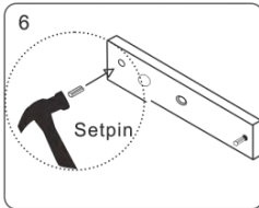
6 Strike the pin into the armature plate slightly (to avoid movement).
