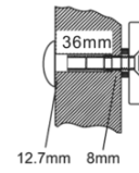
Drill a hole Inside: Diameter is 8mm Outside: Diameter is 12.7mm
