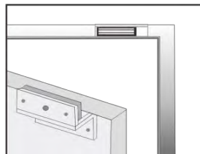
12 Close the door to test holding force. The angle between armature plate and magnetic lock can be adjusted by adding or reducing washers.
