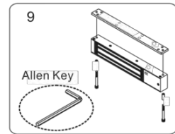
9 Use Allen key to remove the mounting plate from lock body.
