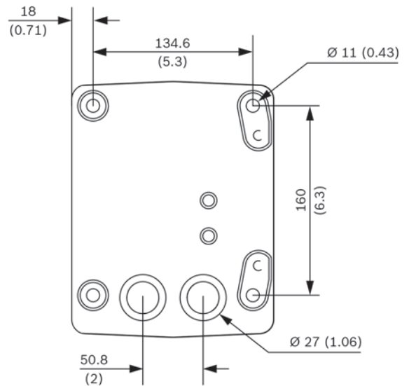
Fig. 8: NDA-U-WMP Wall mount plate
