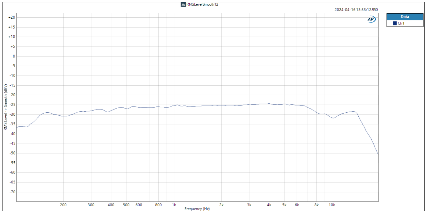
Frequenzgang
